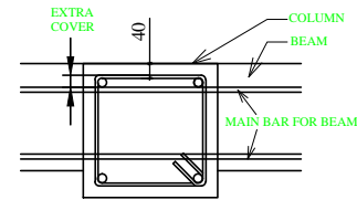
DETAILS FOR EXTRA COVER TO BEAMS
