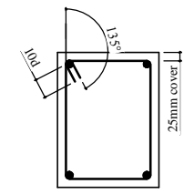
TYPICAL BEAM STIRRUPS DETAILS
