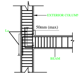
TYPICAL BEAM BAR ANCHORAGE DETAIL
