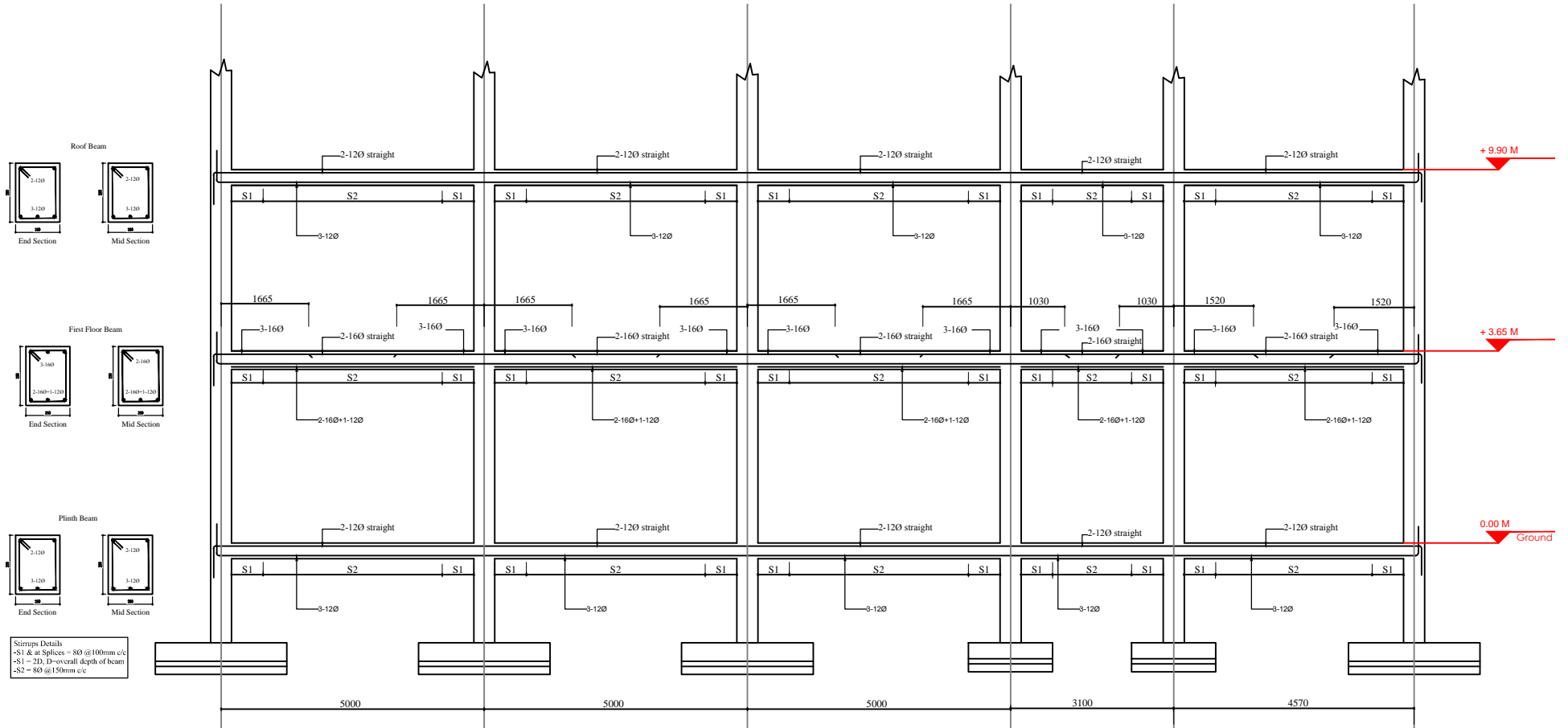
BEAM ALONG GRID - 1, 2, 3 (1st, 2nd & ROOF FLOOR)
