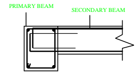
PRIMARY AND SECONDARY BEAM JUNCTION DETAILS
