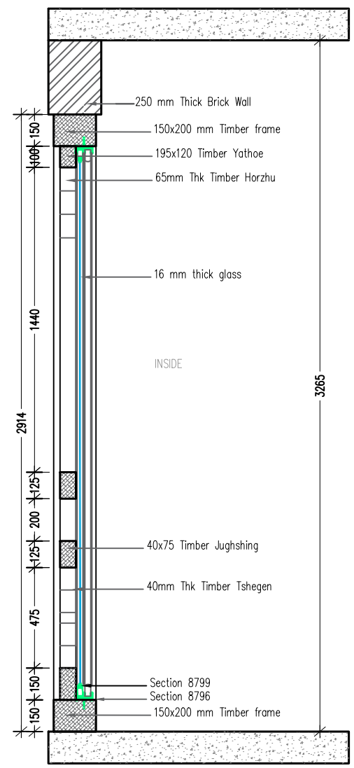
SECTION 1-1
