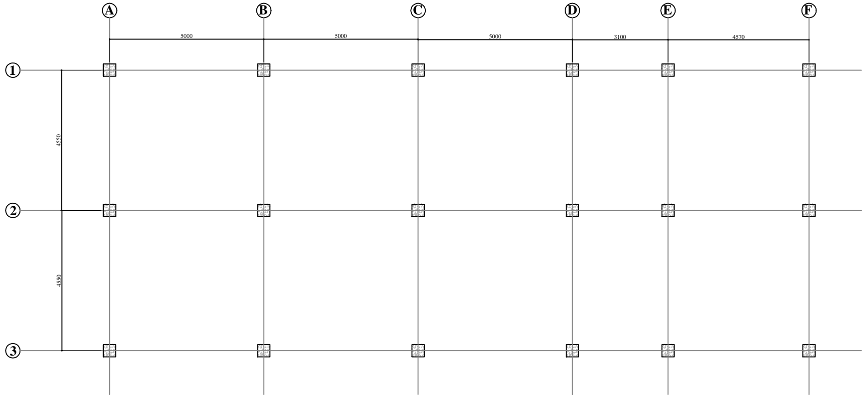
(250X250), COLUMN LAYOUT PLAN
