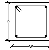
RECTANGULAR TIES DETAIL OF COLUMN
