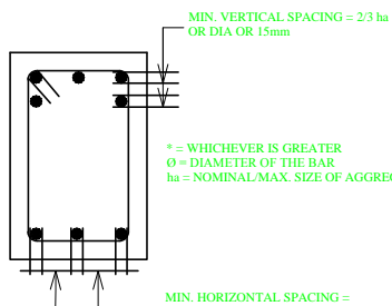
TYPICAL DETAILS FOR MINIMUM CLEARANCE BETWEEN INDIVIDUAL BARS
