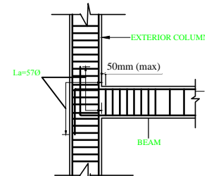
EXTERIOR BEAM-COLUMN JUNCTION DETAIL
