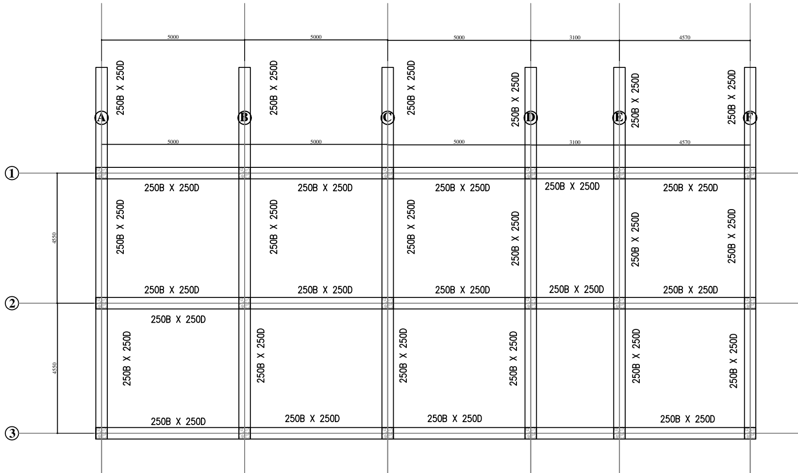
FIRST FLOOR BEAM LAYOUT PLAN
