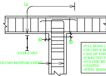
COLUMN TERMINATION DETAILS IN BEAM (ELEVATION)
