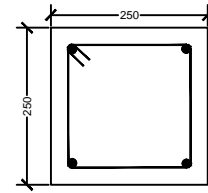
ARRANGEMENT OF 8-20Ø REBARS FOR C1 (400x400)
