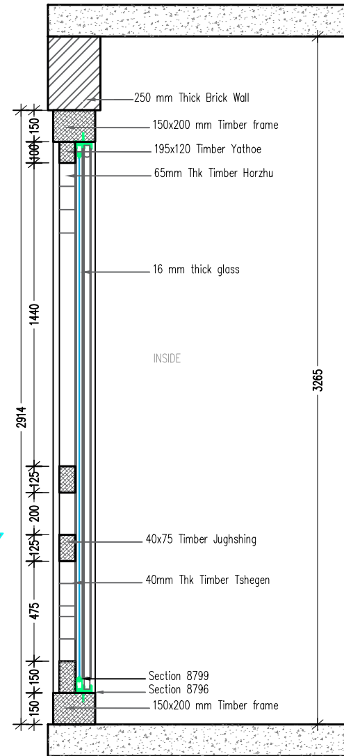
SECTION 1-1
