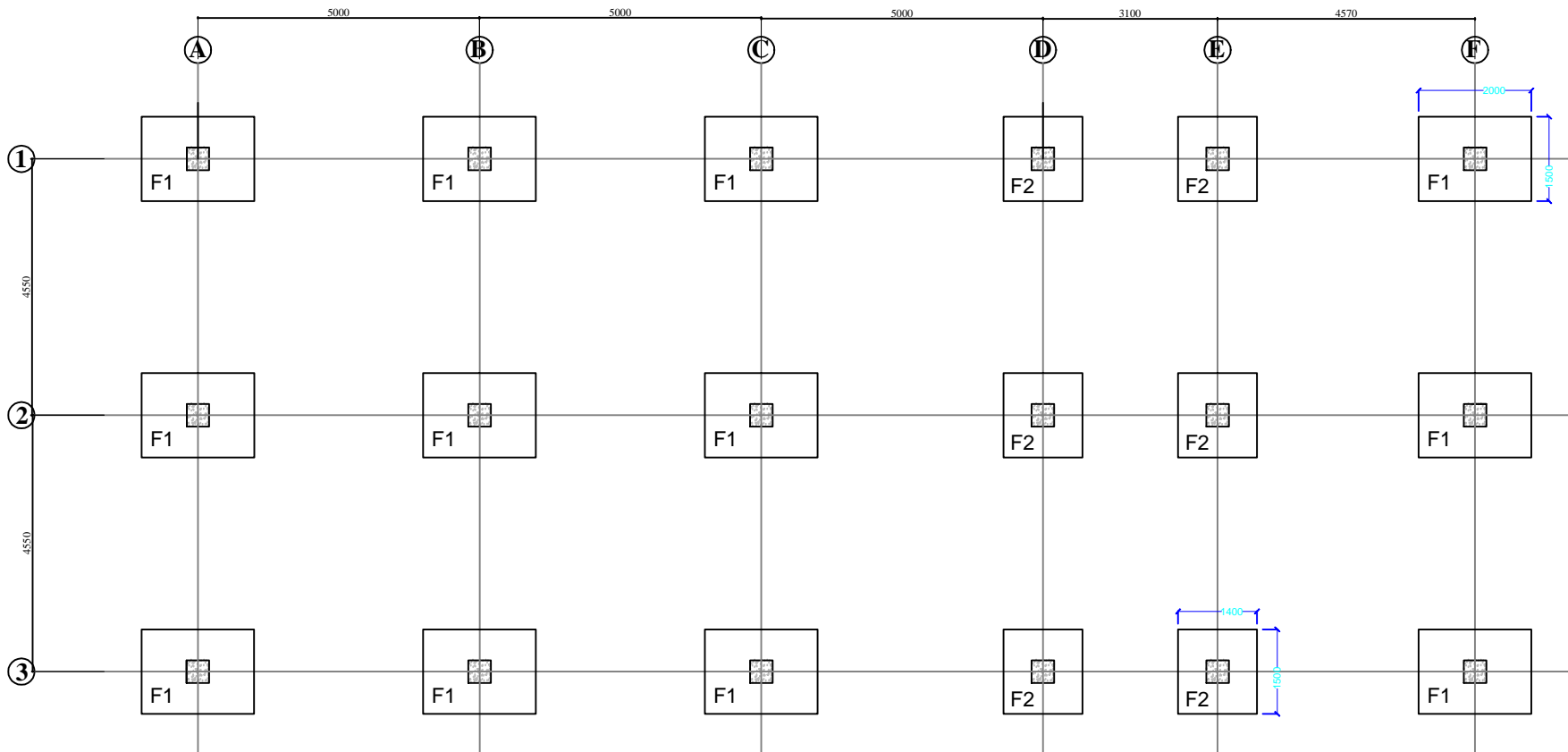
FOOTING LAYOUT PLAN
