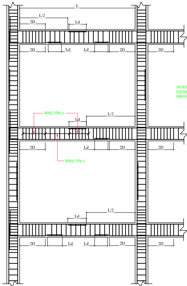
TYPICAL ARRANGEMENT OF STIRRUPS & SPLICES IN BEAMS
