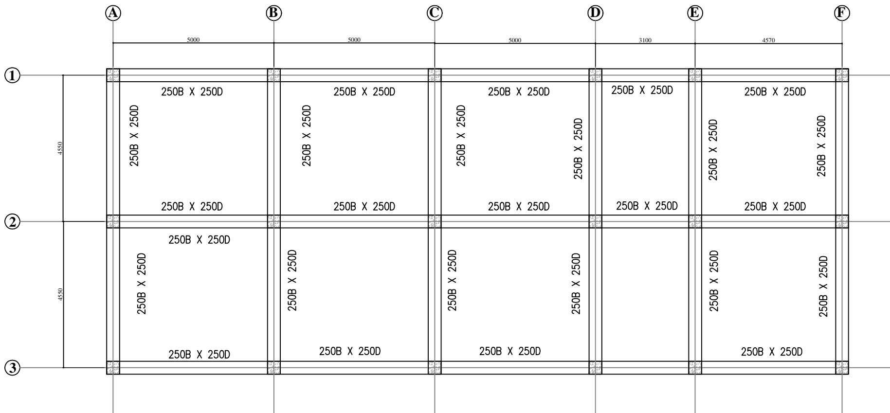
PLINTH BEAM & ROOF BEAM LAYOUT PLAN
