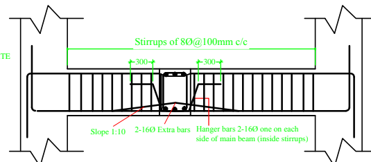
PRIMARY AND SECONDARY BEAM CONNECTION DETAILS
