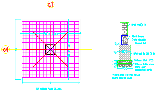
FOOTING DETAILS
