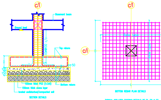
TYPICAL ISOLATED FOOTING DETAILS OF F1, F2 & F3
