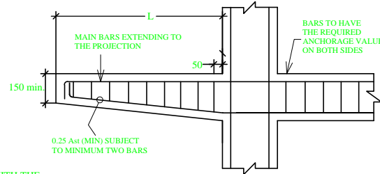
TYPICAL CANTILEVER BEAM DETAILS PROJECTING FROM BEAM OR COLUMN
