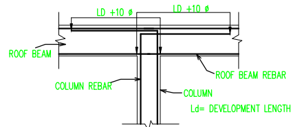
COLUMN REBARS ANCHORAGE DETAILS AT THE ROOF
